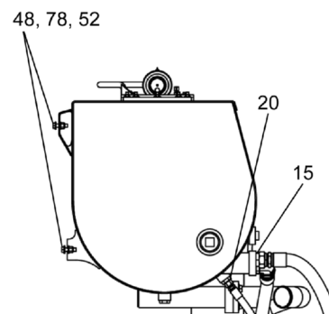
VIEW K-K
