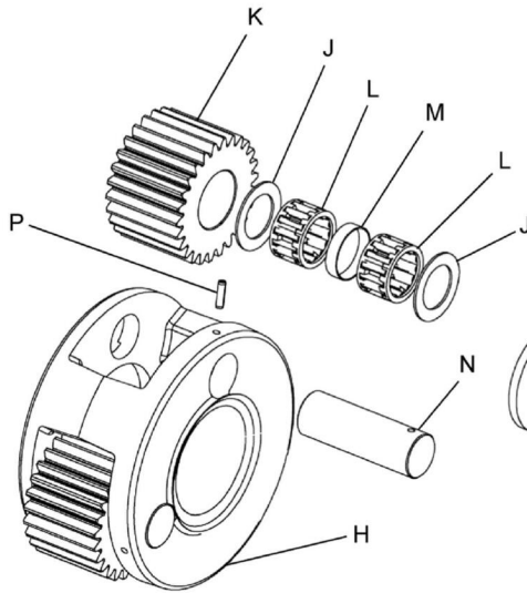
OUTPUT PLANET ASSEMBLY
