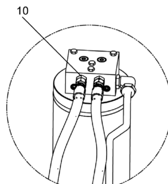
DETAIL P
