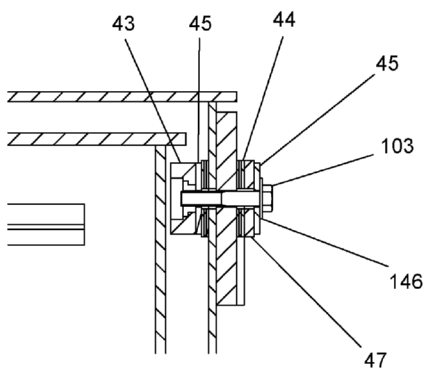
SECTION G - G
