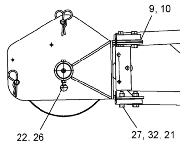
VIEW B - B
