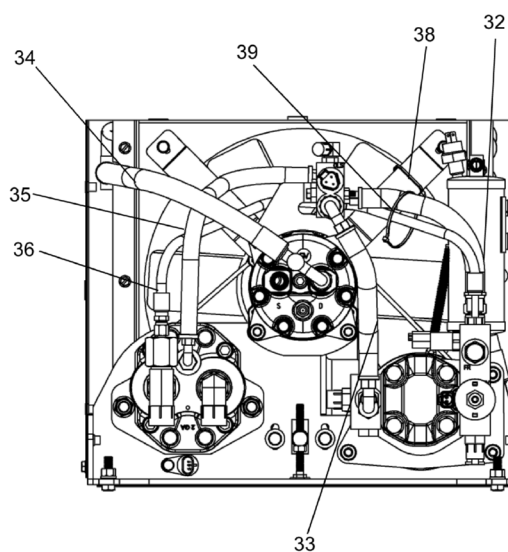
ASSY STAGE 3
