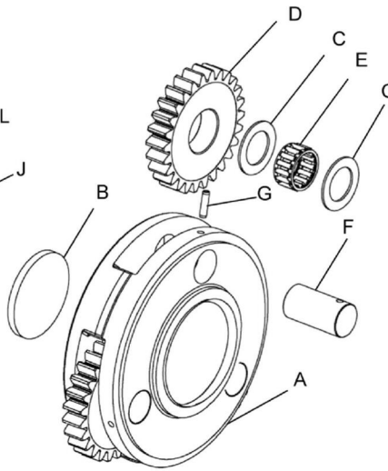
PRIMARY PLANET ASSEMBLY
