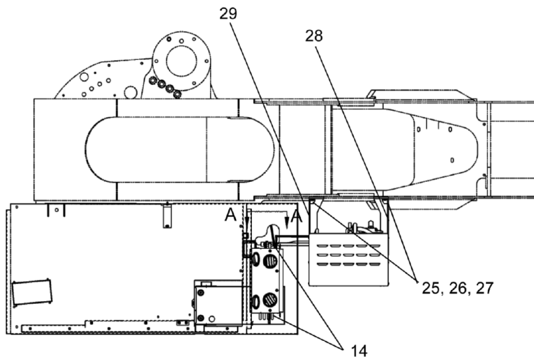
MOUNTING DETAIL OF CAB BLOWER AND HYD. A/C UNIT
