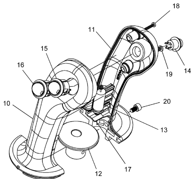
HANDLE ASSEMBLY
