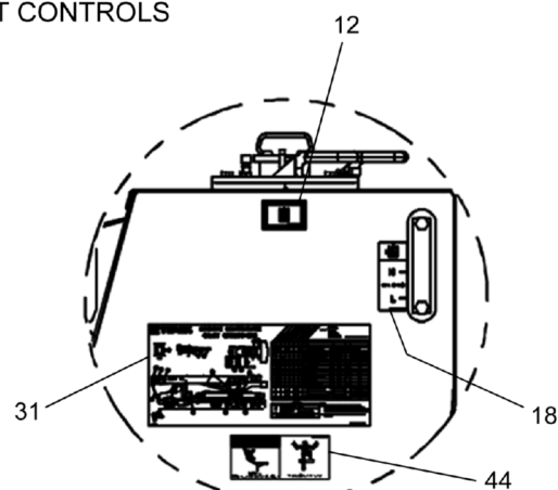
DETAIL A HYDRAULIC TANK
