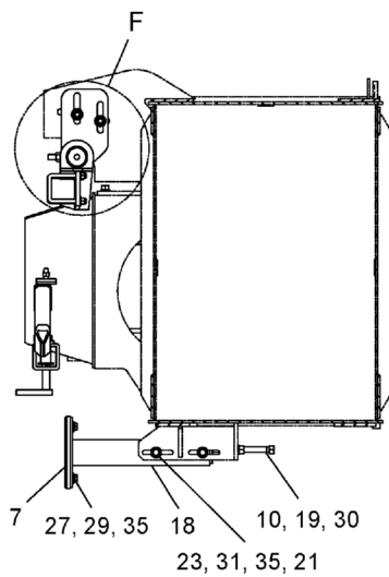
VIEW D - D
