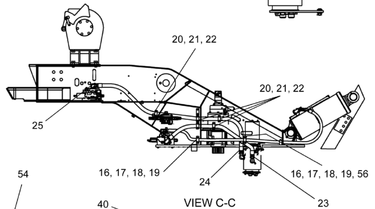
VIEW C-C
