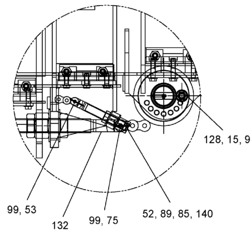
DETAIL L
