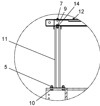
DETAIL C
