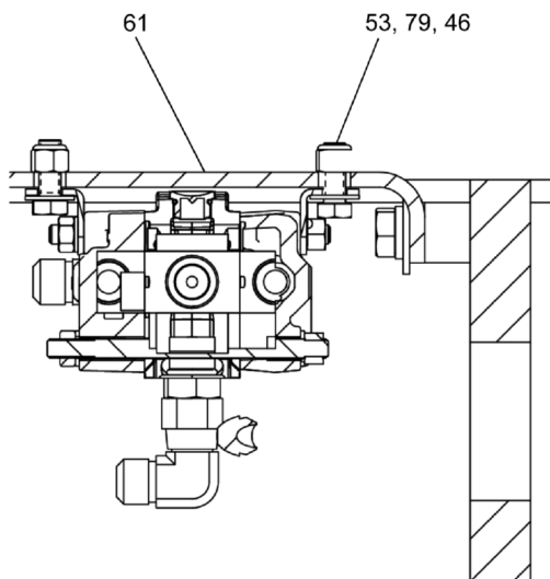
SECTION M-M
