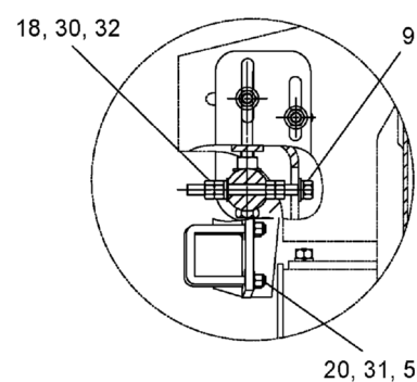
DETAIL G
