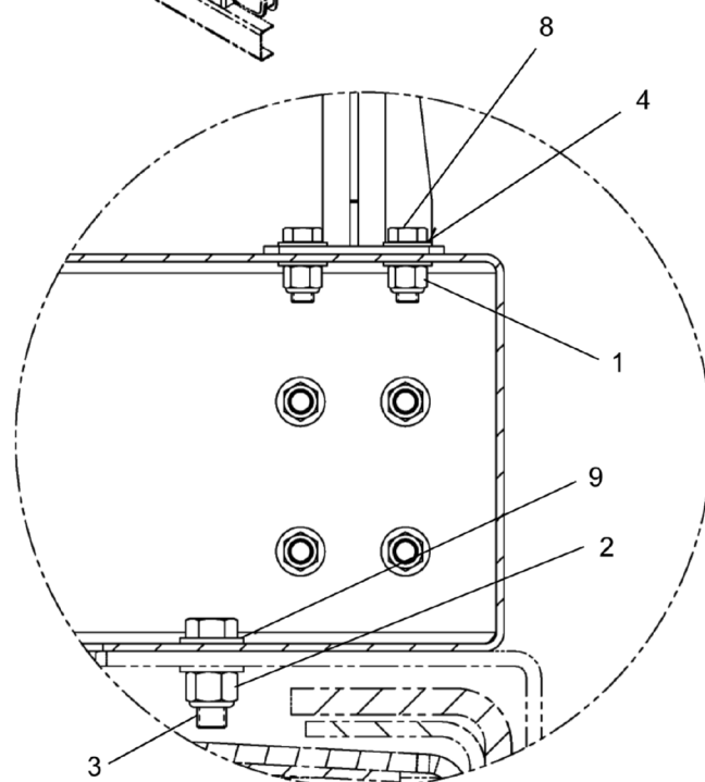
DETAIL B
