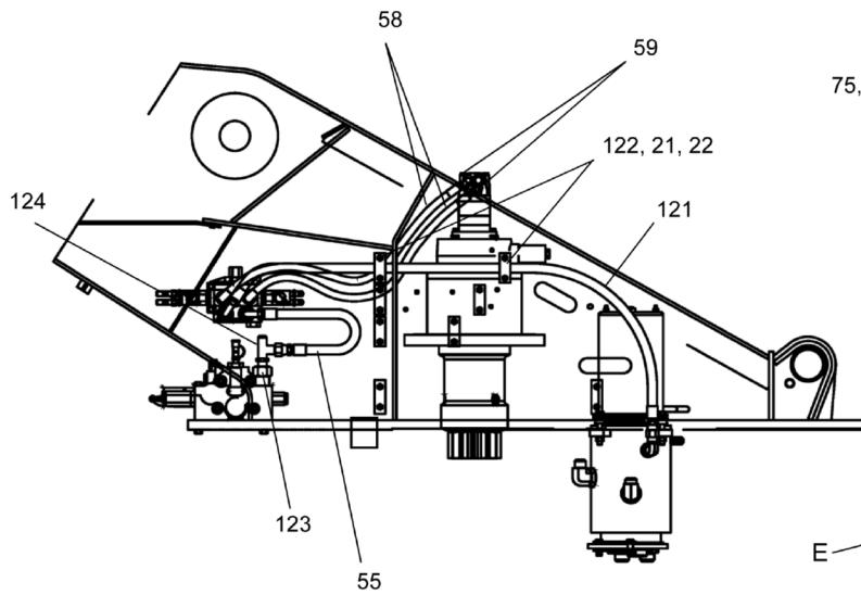
PLUMBING FOR THE FRONT FACE OF SWING VALVE
