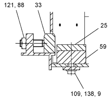
SECTION H - H
