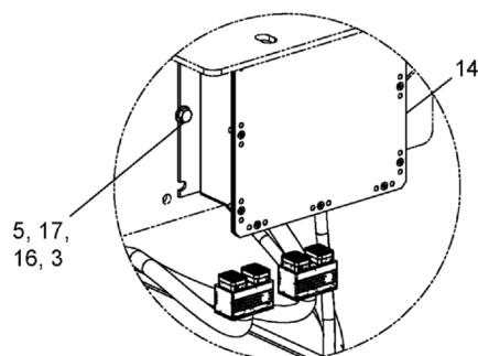
DETAIL F
