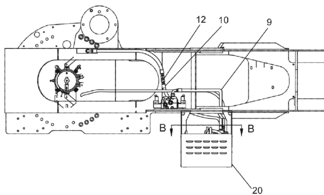
MOUNTING DETAIL OF CAB BLOWER AND HYD. A/C UNIT
