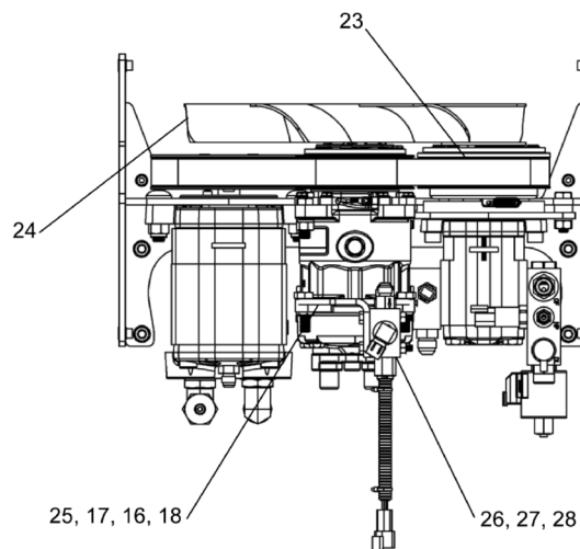
ASSY STAGE 3
