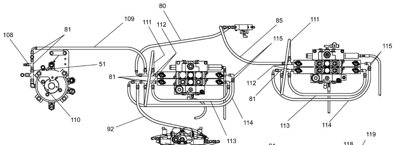
BOOM WINCH & SWING VALVE PILOT DRAINS
