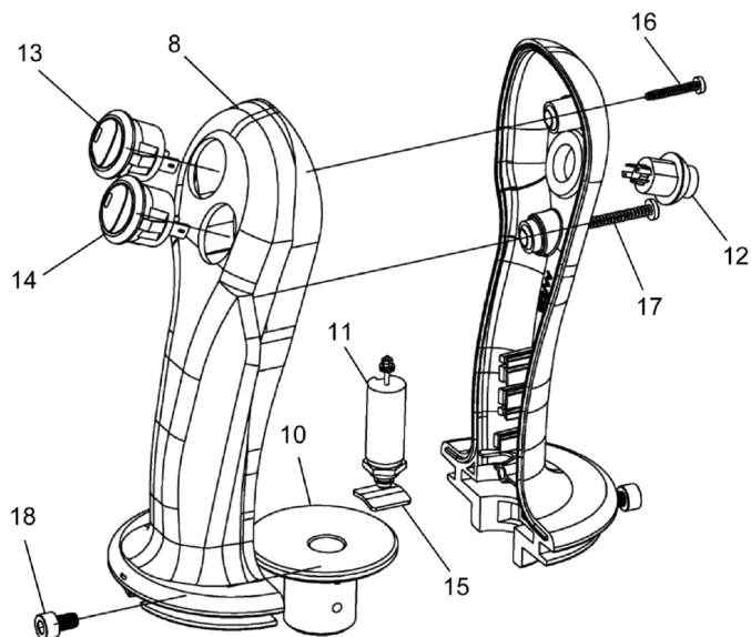
HANDLE ASSEMBLY
