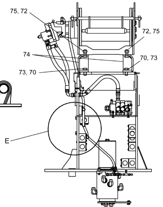
PLUMBING FOR THE FRONT FACE OF SWING VALVE
