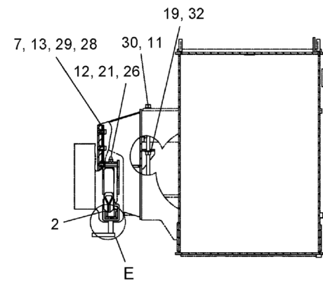
VIEW C - C
