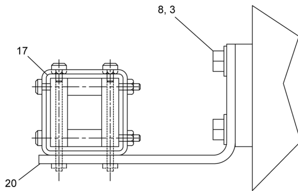
SECTION C - C
