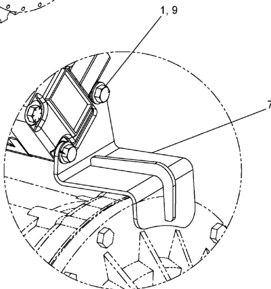
DETAIL A
