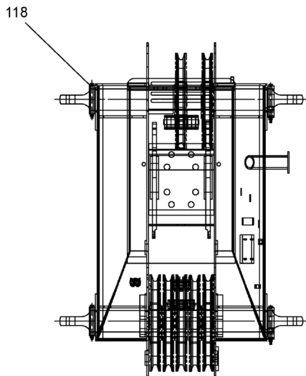
5 SHEAVE HEAD OPTION
