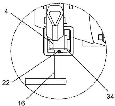
DETAIL F
