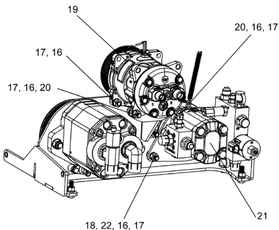
ASSY STAGE 2
