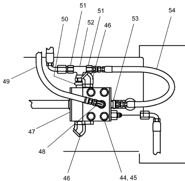
VIEW B-B
