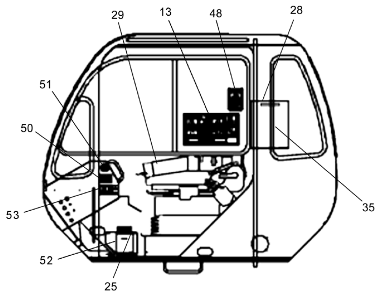
INTERIOR DETAIL OF UPPER CAB
