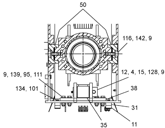
SECTION N - N
