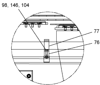
DETAIL M
