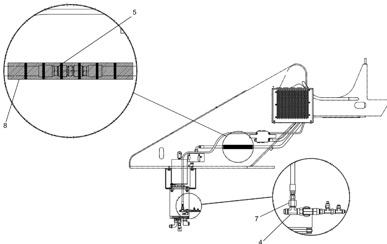
DETAIL OF A/C TO CAB HOSES AND ELECTRICAL WIRING
