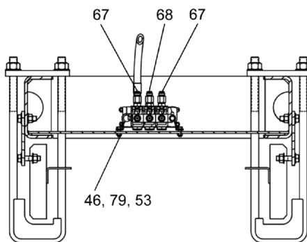
SECTION F-F
