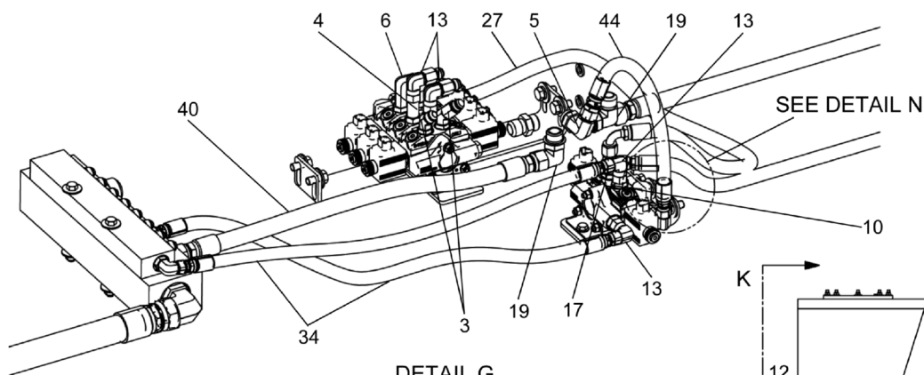
DETAIL G
