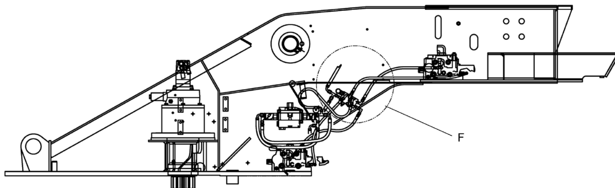
DETAIL OF BOOM, WINCH & SWING VALVE PILOT/SUPPLY PLUMBING
