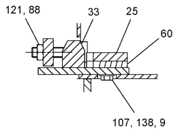
SECTION F - F
