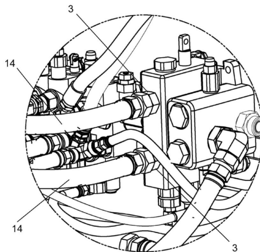
DETAIL F
