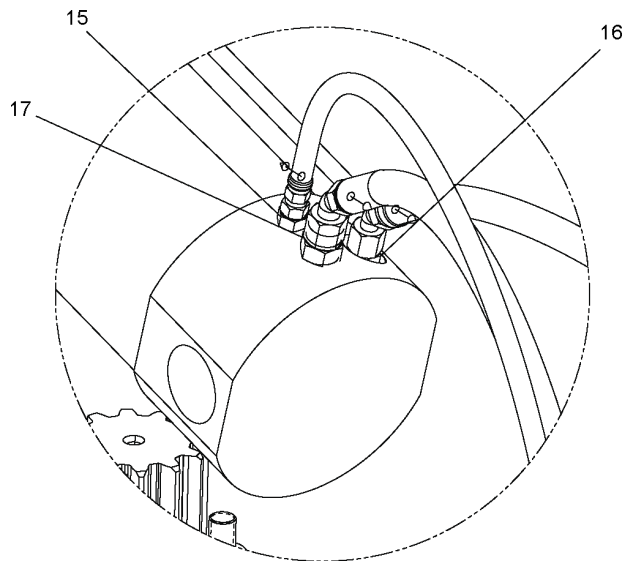
DETAIL J
