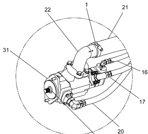
DETAIL C
