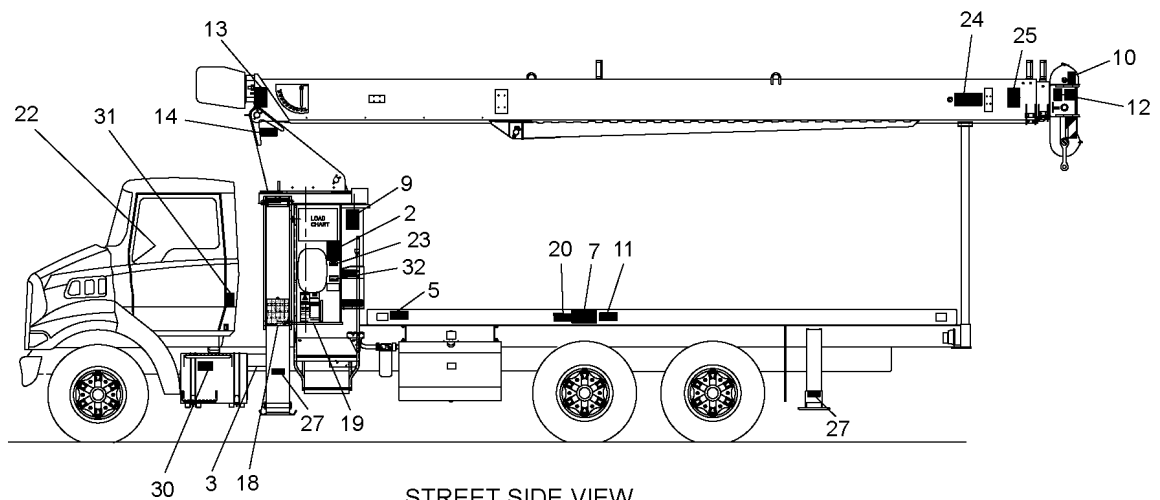
STREET SIDE VIEW
