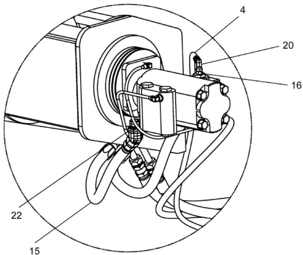
DETAIL E
