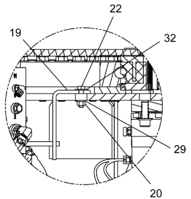
DETAIL G
