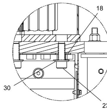
DETAIL H
