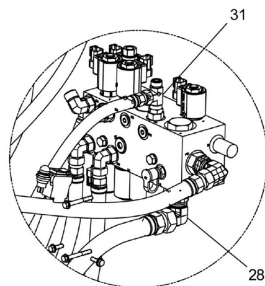
DETAIL J
