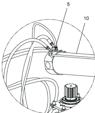
DETAIL C
