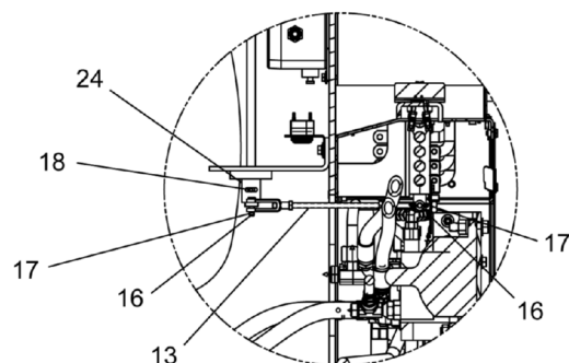
DETAIL L
