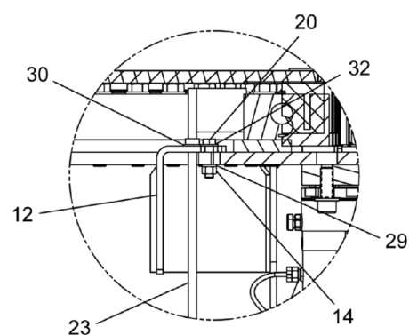
DETAIL M
