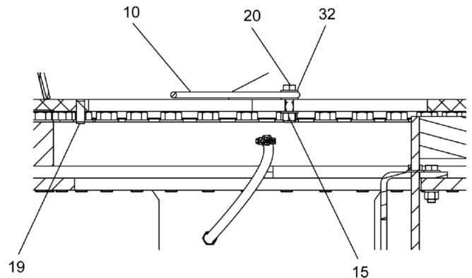
SECTION J - J
