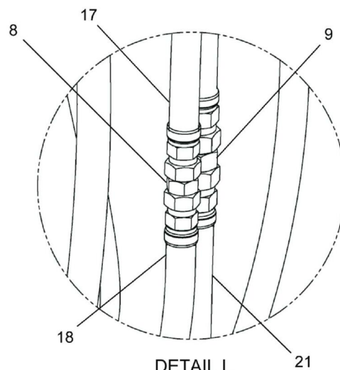
DETAIL L
