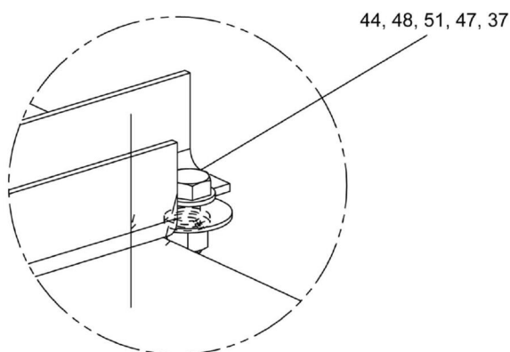
DETAIL M
