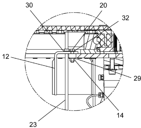
DETAIL G
