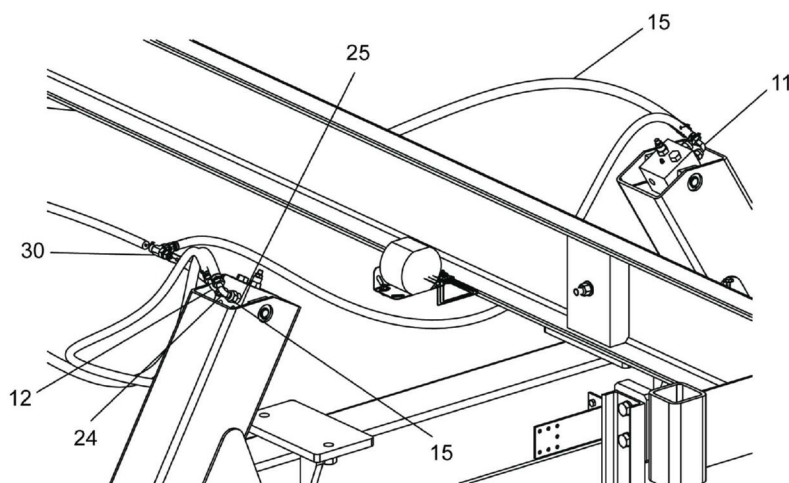
DETAIL J
