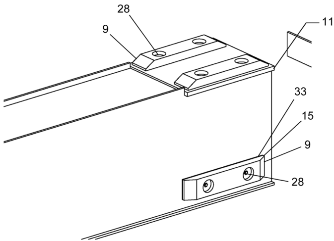
VIEW F
