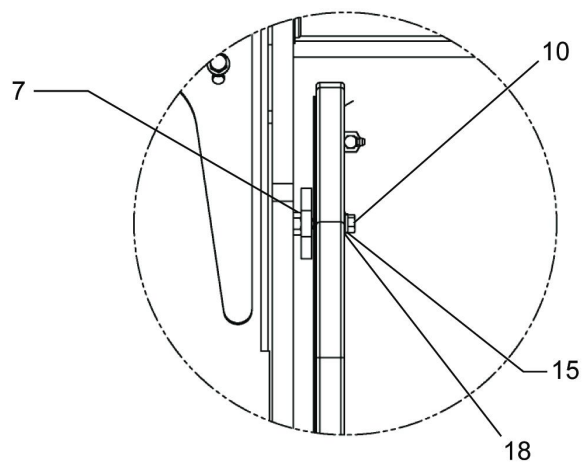
DETAIL E
