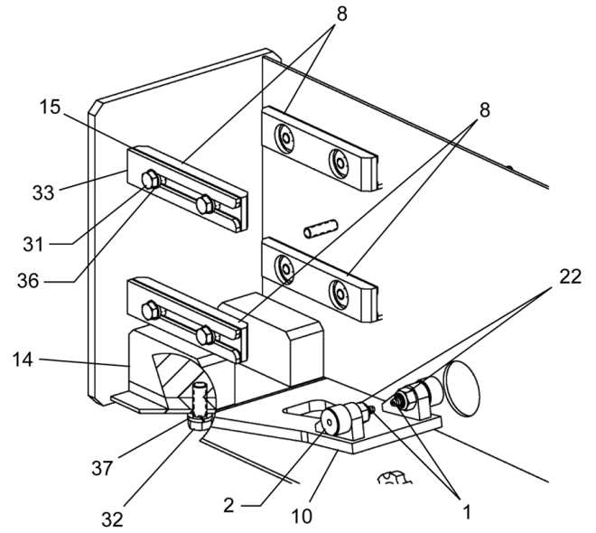
VIEW E
