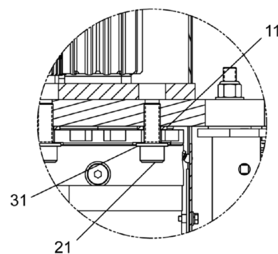
DETAIL N
