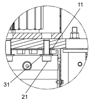
DETAIL H
