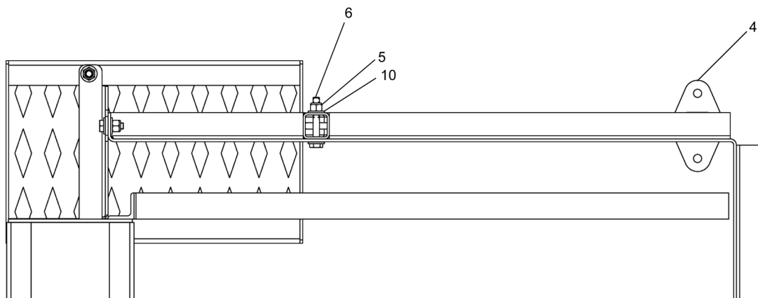
BOTTOM VIEW
