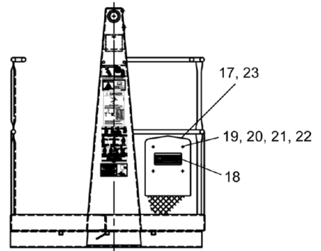
VIEW B-B
