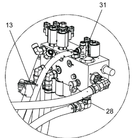
DETAIL G
