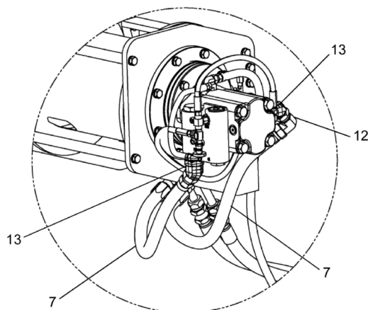
DETAIL E
