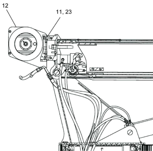
SECTION M-M
