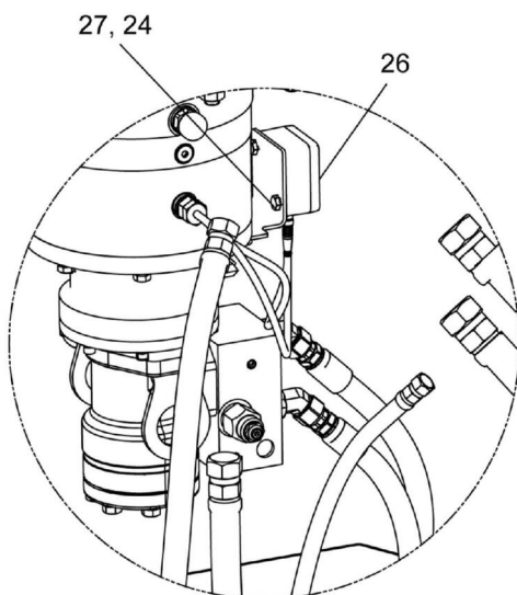
DETAIL B
