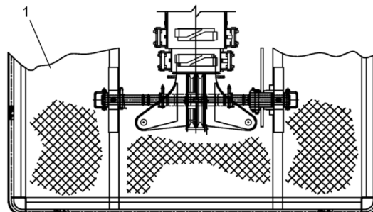
BOOM TOP VIEW
