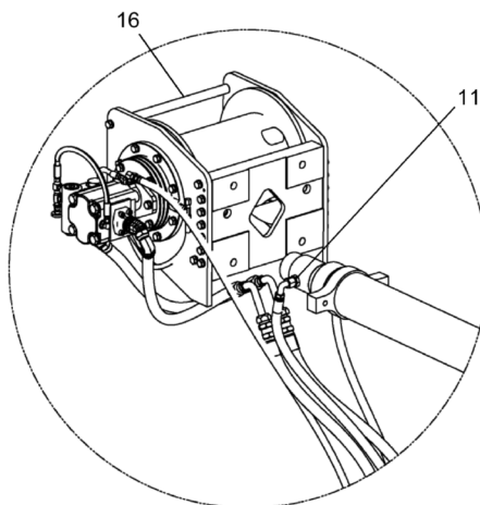
DETAIL C
