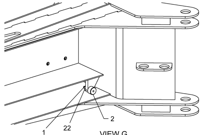
VIEW G
