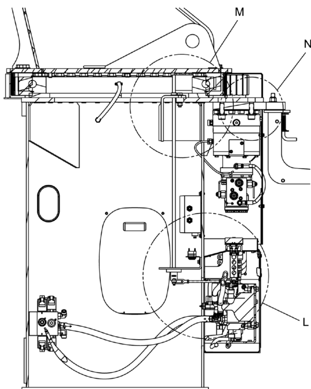
SECTION K - K
