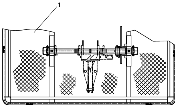
JIB INSTALLATION TOP VIEW
