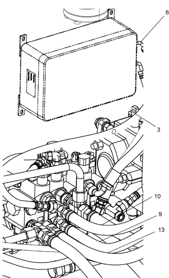
DETAIL K
