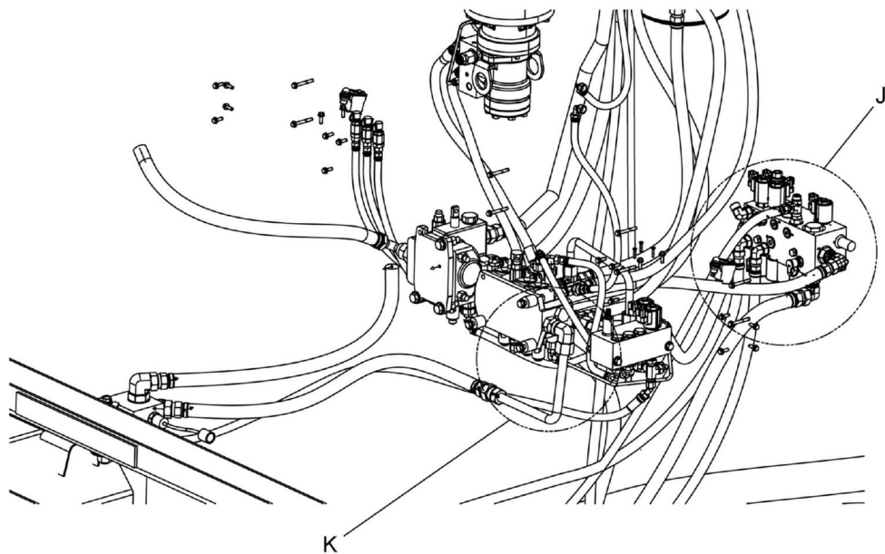
VIEW H - H
