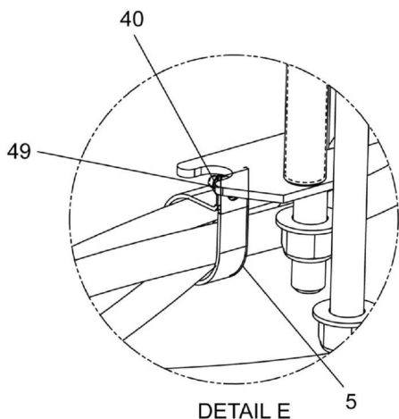
DETAIL E
