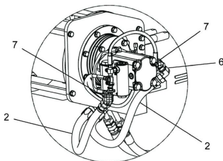
DETAIL E
