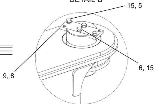
DETAIL C
