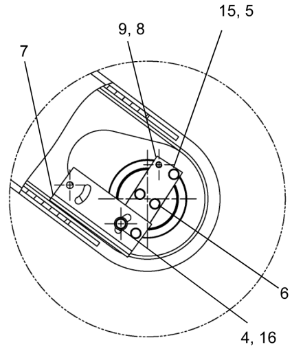
DETAIL H
