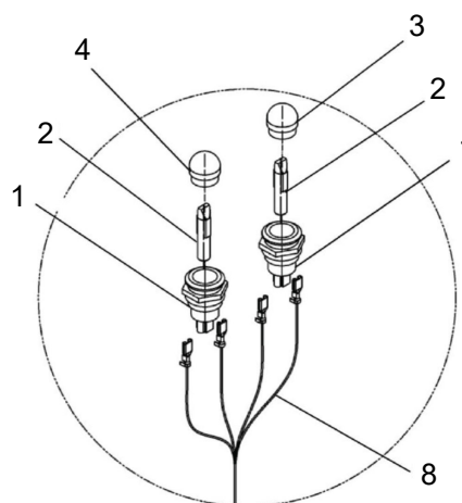
DETAIL C
