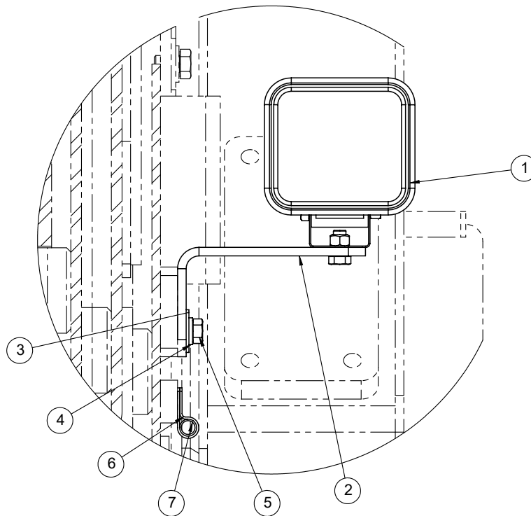
DETAIL A
