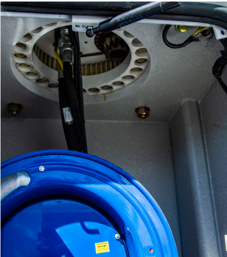
Sealed crane compartment design eliminates drain pan system. Crane mounting structure eliminates the load into the body.
